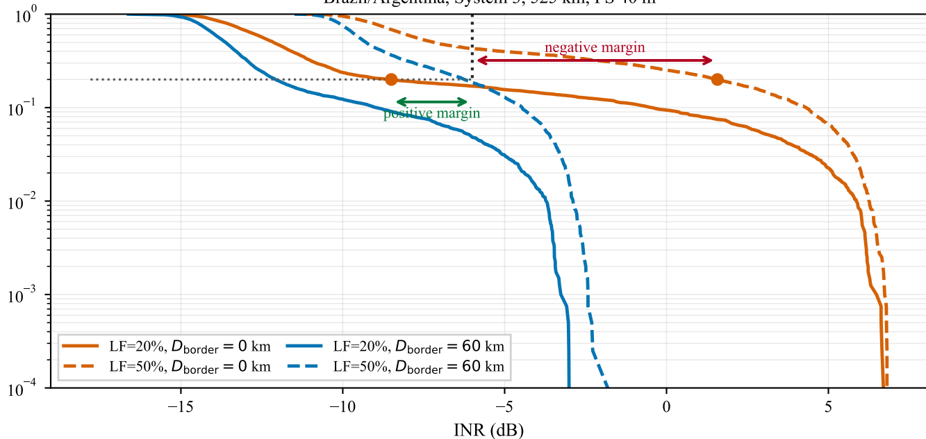
Brazil/Argentina, System 3, 525 km, FS 40 m
